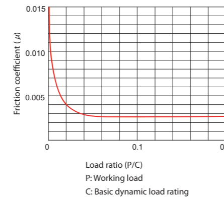
Relationship between working load and friction coefficient.
